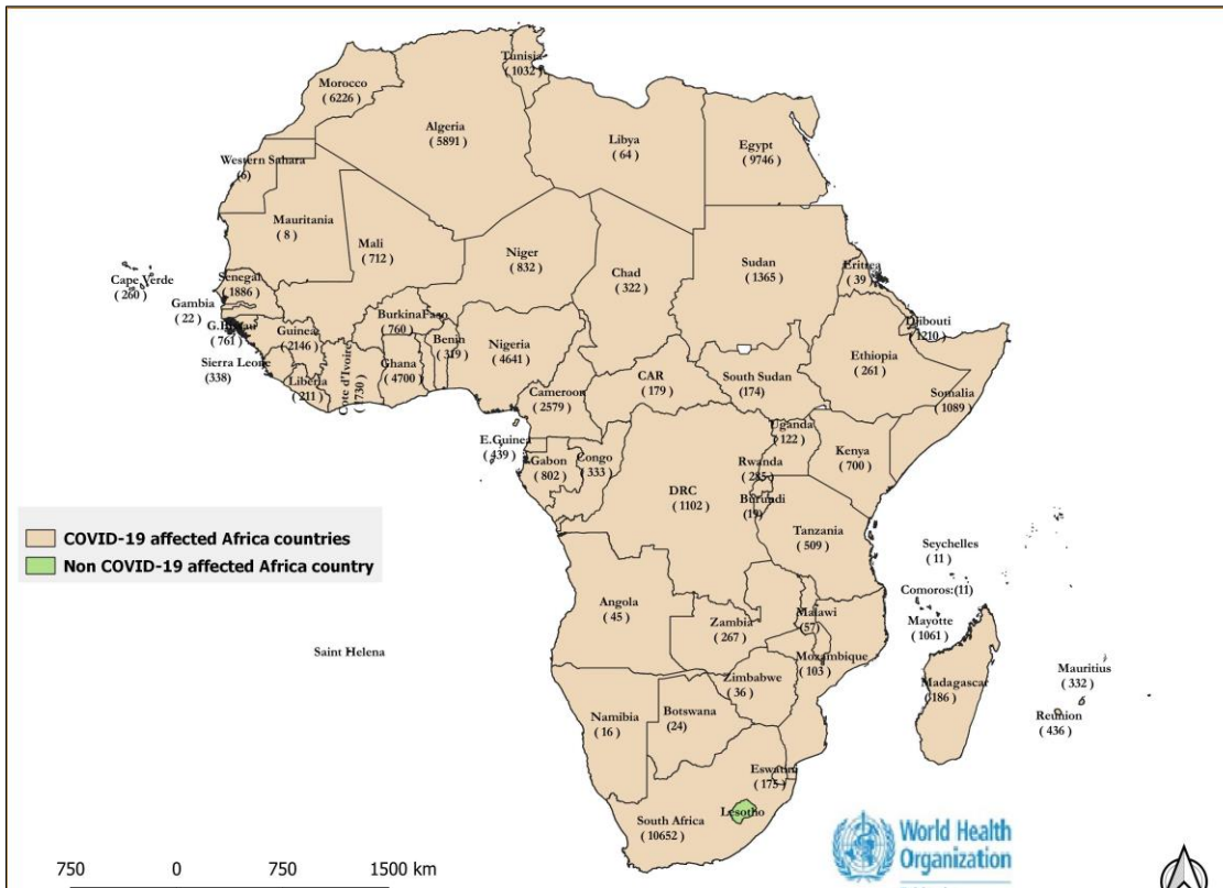
Fig. 1: Map of Africa showing confirmed COVID-19 cases, 12-May 2020
