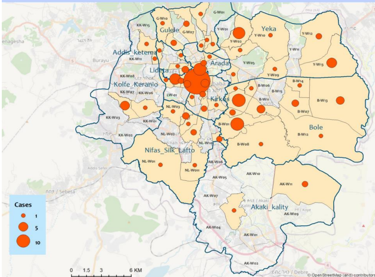
Distribution of Confirmed cases of COVID-19, Addis Ababa, 12 May 2020
