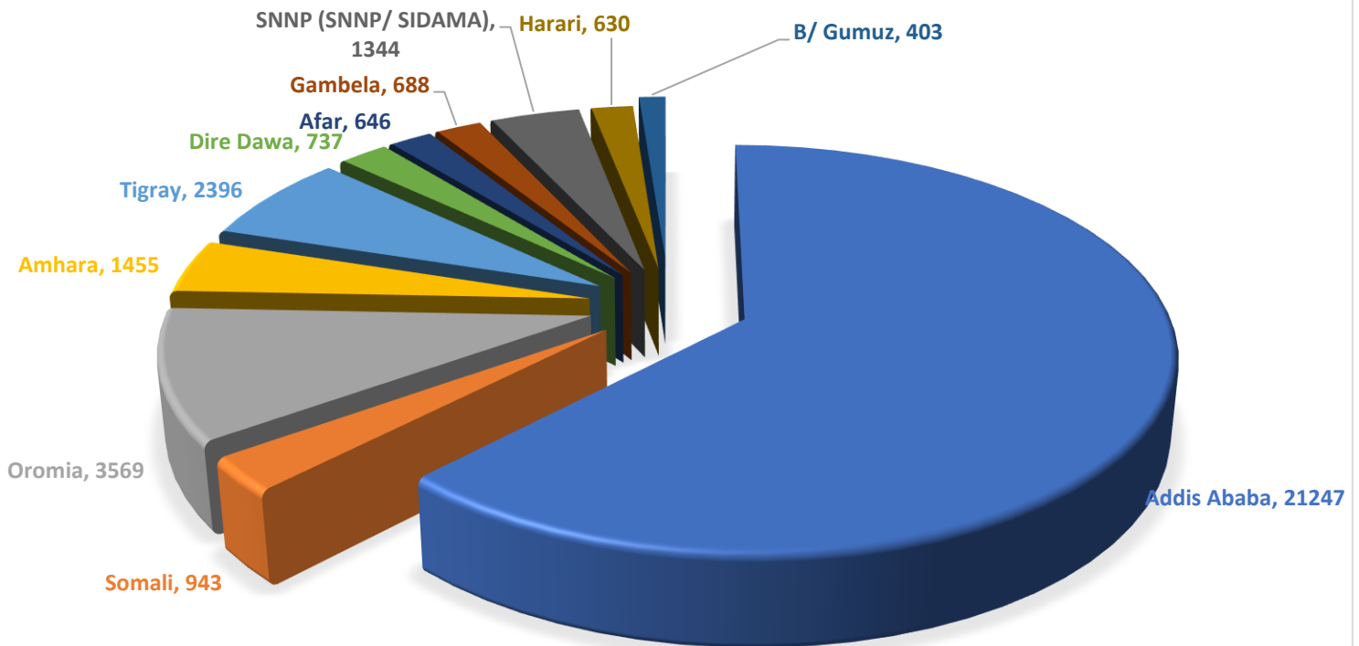
Fig 4: Total confirmed coronavirus cases in various regions of Ethiopia; 19 August 2020
