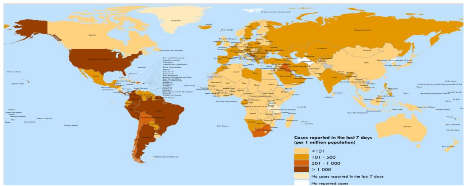
Fig 2: The summary of coronavirus within the five African regions; 19 August 2020
