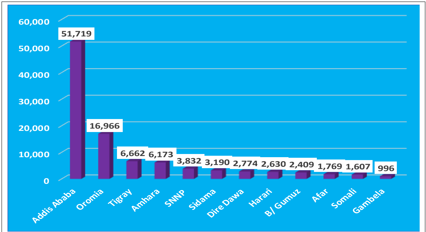
Fig. 4: Distribution of cumulative confirmed COVID-19 cases across the regions, Ethiopia; 11-Nov-2020
