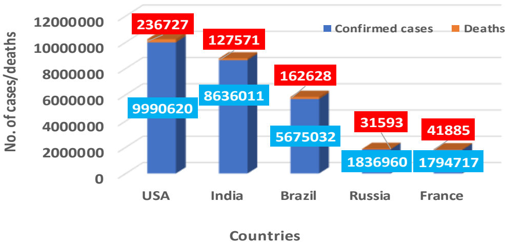
Fig. 1: Top five countries with the highest number of confirmed COVID-19 cases; 11-Nov-20
