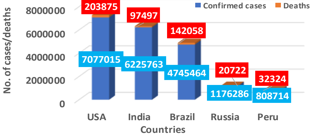
Fig. 1: Top five countries with the highest number of confirmed COVID-19 cases; 30-Sep-20
