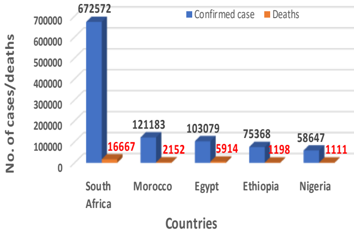
Fig. 2: Five countries with the highest number of confirmed COVID-19 cases on the African continent; 30-Sep-2020
