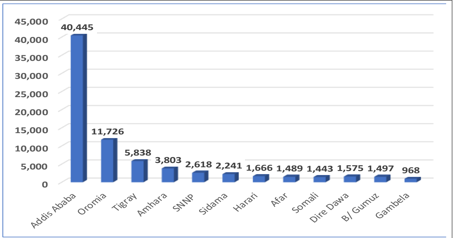
Fig. 5: Total confirmed COVID-19 cases per region in Ethiopia, 30-Sep 2020
