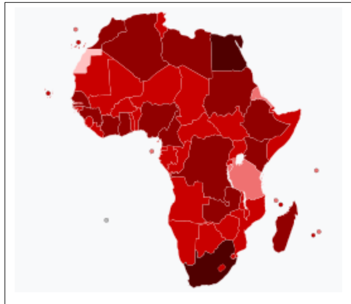
Fig. 3: Confirmed COVID-19 cases in Africa; 30-Sep-2020
